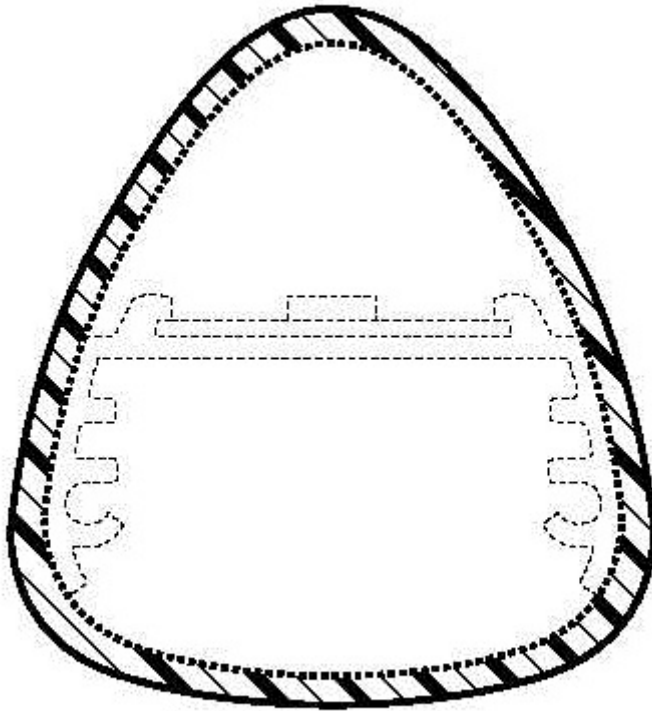
CROSS-SECTIONAL VIEW TAKEN ALONG LINE 8-8 IN FIGURE 1A
